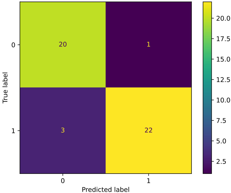
Confusion Matrix for Weighted Ensemble Model
